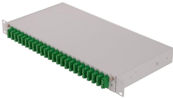
TMVJ-1U with FT-24-SC base unit with front panel for 24x SC adapters
